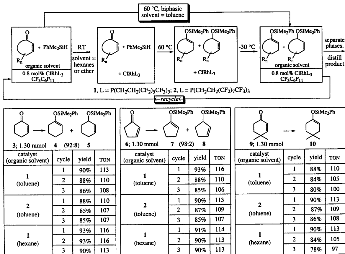
Figure 1. Fluorous rhodium-catalyzed hydrosilylation: biphasic and monophasic conditions
